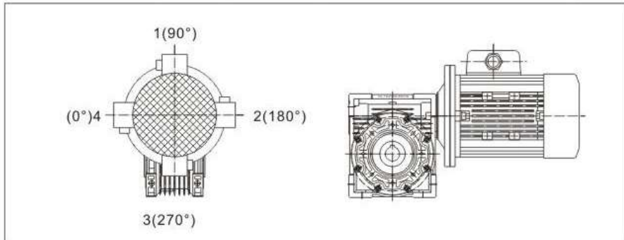
电机接线盒位置(从电机风扇罩向输出端看) Motor thermal box position(viewed output shaft from fan cowl of motor)
