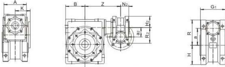
组合型二级蜗杆减速器外形尺寸图 Diagram for double-stage worm reducer combination
