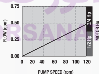
EP2006 Performance
